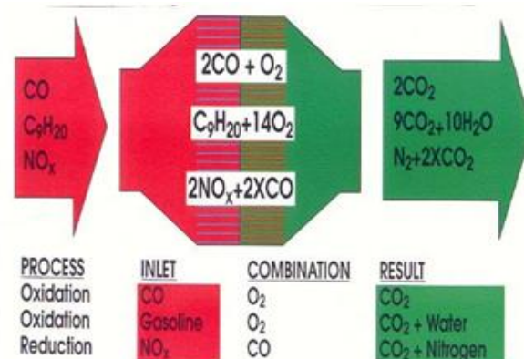
Fig 3: The catalytic converter is an essential component of the chemical system that reduces the amount of pollutants caused by automobile exhaust.
