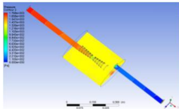
Figure 4- 4 Design 3's pressure curve is being studied.
