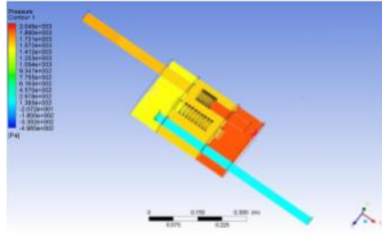
Figure 4- 5 The pressure shape of design 4 is depicted in the image below.
