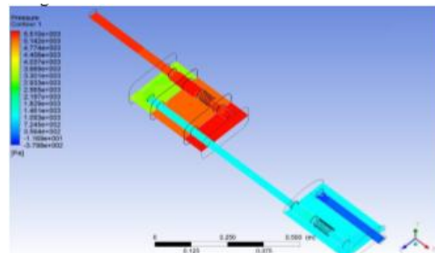
Figure 4- 7 In Design 6, the pressure curve is depicted.
