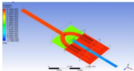
Figure 4- 2 Design 1's pressure curve is being studied.
