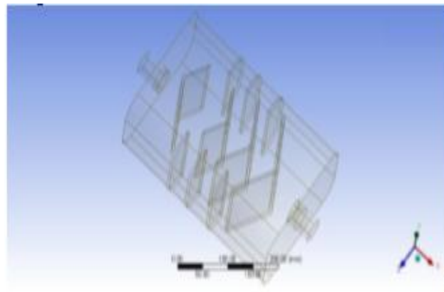
Figure 3-5 This research provides a three-dimensional assessment of Design 2.
